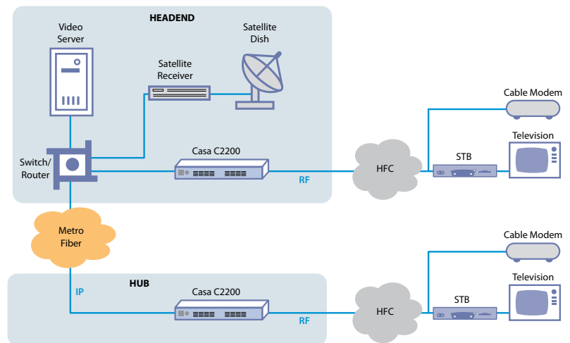
C2200 Application Diagram
